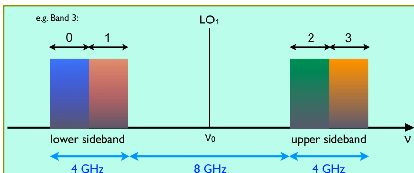
Figure 34: A graphical view of basebands and sidebands. Basebands may be tuned to overlap if the user wishes, or may be located so as to maximize the total bandwidth (as shown). Each baseband may be further subdivided into as many as 8 spectral windows. Up to four spectral windows per baseband are available.
