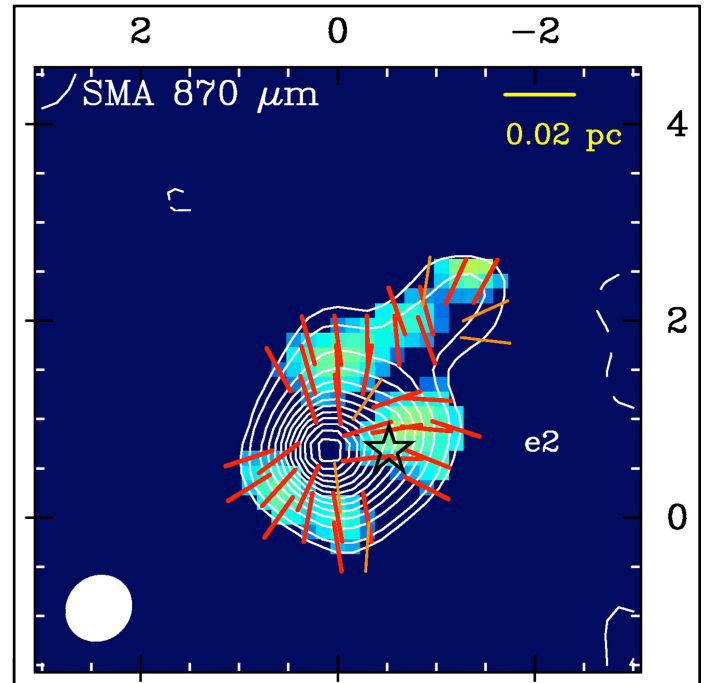
Figure 22: Magnetic field of the W51 e2 core at 0.9 mm obtained at the Submillimeter Array. The total intensity is shown in contours. The polarization intensity is shown in color scale. The star denotes the ultracompact HII region. (Credit: Ya-Wen Tang, 2009 ApJ, 700, 251)
