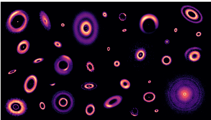
Figure 21: “Freshly baked dust doughnuts from our local cosmic café”. This image, a finalist in NSERC-Canada’s Science Exposed 2021 photo contest, shows 37 images of dust disks around nearby young stars observed by ALMA. The unseen young planets can sculpt the disk into a beautiful structure of rings and arcs as they carve gaps along their orbits. (Credits: L. Francis; N. van der Marel)
