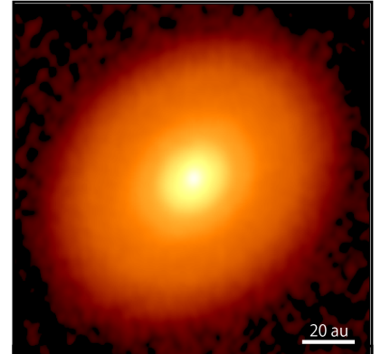
Figure 20: In contrast to the images shown in Figure 21 (below), this high resolution Band 7 image of the protoplanetary disk around DG Tau shows a very smooth appearance, absent of ring-like structures, indicating a phase shortly preceding planet formation. (Credits: ALMA (ESO/NAOJ/NRAO); S. Ohashi et al., 2023, ApJ, 954, 110)
