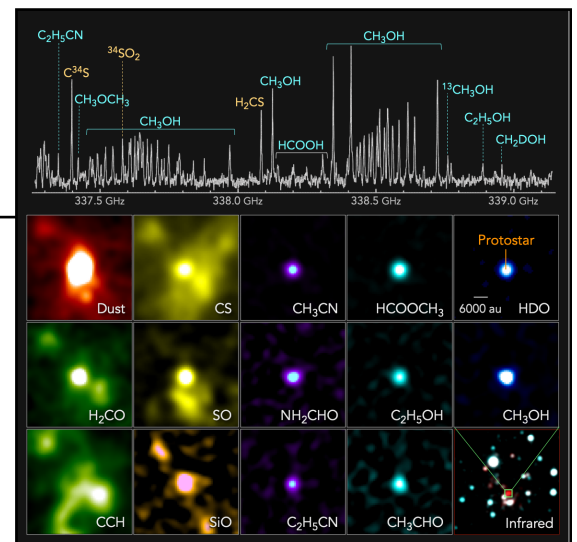
Figure 33: Top: Band 7 spectrum of a protostar, WB 89-789, located in the extreme outer Galaxy. Bottom: Distributions of radio emissions from the protostar. Emissions from dust, formaldehyde (H 2 CO), ethynylradical (CCH), carbon monosulfide (CS), sulfur monoxide (SO), silicon monoxide (SiO), acetonitrile (CH 3 CN), formamide (NH 2 CHO), propanenitrile (C 2 H 5 CN), methyl formate (HCOOCH 3 ), ethanol (C 2 H 5 OH), acetaldehyde (CH 3 CHO), deuterated water (HDO), and methanol (CH 3 OH) are shown as examples. Bottom right panel, an IR 2-color composite image of the surrounding region is shown (red: 2.16 \mu and blue: 1.25 \mu , based on 2MASS data). (Credit: ALMA (ESO/NAOJ/NRAO), T. Shimonishi (Niigata University))
