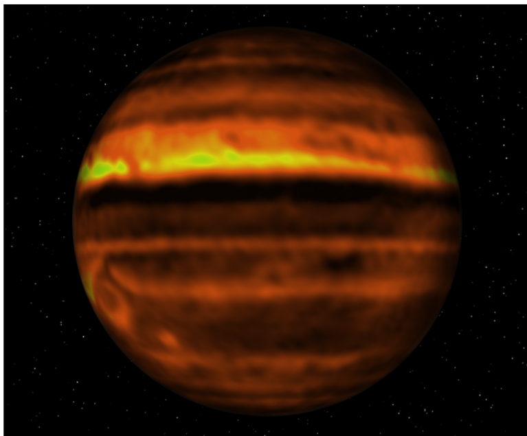
Figure 28: Spherical image of Jupiter showing the distribution of ammonia gas below Jupiter's cloud deck. (Credit: ALMA (ESO/NAOJ/NRAO), I. de Pater et al.; NRAO/AUI NSF, S. Dagnello)
