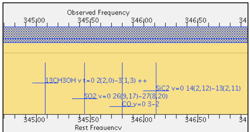
Figure 39: Four spectral windows were set up to observe these four lines simultaneously in one baseband using the OT. The windows are each 234 MHz wide (with 0.43 km/s channels), and are centered at 345.80, 345.45, 346.11 and 345.09 GHz. The spectral windows must fit within the 2 GHz wide baseband.
