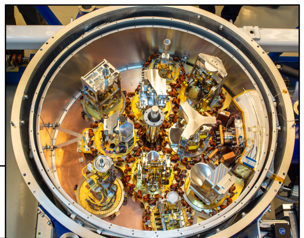
Figure 36: An open cryostat fitted with receivers covering Bands 1 through 10, including the prototype Band 2 cartridge. When fully populated, ALMA will have complete coverage available from the ground from 35 GHz to 950 GHz. (Credit: ALMA (ESO/NAOJ/NRAO); Sergio Otarola)
