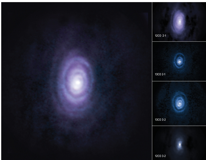
Figure 25: Composite images of the evolved carbon rich star V Hya showing six slowly expanding rings forming as the star expels its matter. Shown here in composite, these outflowing rings and the diffuse arc structure of the sixth ring are moderately visible in the ^{12}\text{CO} carbon isotope emission line, and become well-defined in views of the ^{13}\text{CO} carbon isotopes. (Credit: Sahai et al.; ALMA (ESO/NAOJ/NRAO)/S. Dagnello (NRAO/AUI/NSF))
