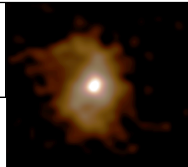
Figure 31: ALMA image of the galaxy BRI 1335-0417 at redshift 4.41. ALMA detected emissions from carbon ions in the galaxy. Spiral arms are visible on both sides of the compact, bright area in the galaxy center. The discovery of a galaxy with a spiral structure at such an early stage (a mere 1.4 billion years after the Big Bang) makes this the earliest known spiral galaxy. (Credits: ALMA (ESO/NAOJ/NRAO), T. Tsukui & S. Iguchi)
