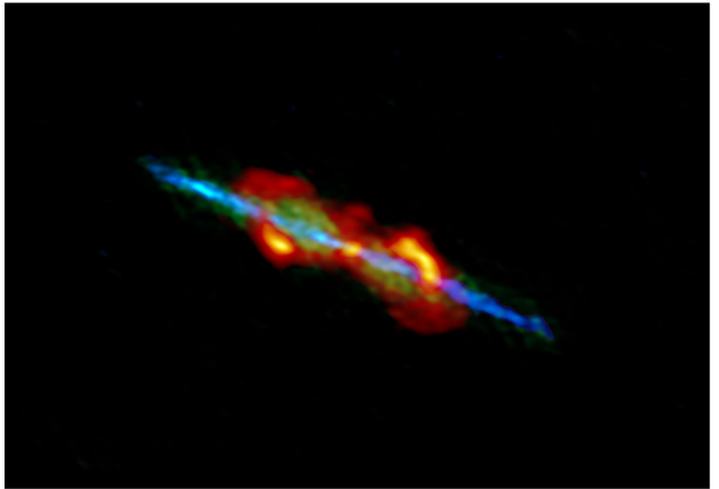
Figure 24: The asymptotic giant branch star W43A was observed by ALMA at Band 6, to understand how bipolar proto-planetary nebulae are generated. Here CO(J=2-1) emission clearly shows a high velocity jet (blue) ejected from the aged central star, within a lower velocity (green), with the dusty envelope of the star entrained by the jets shown in orange. (Credits: ALMA (ESO/NAOJ/NRAO); Tafuya et al., 2020, ApJ, 890, L14)
