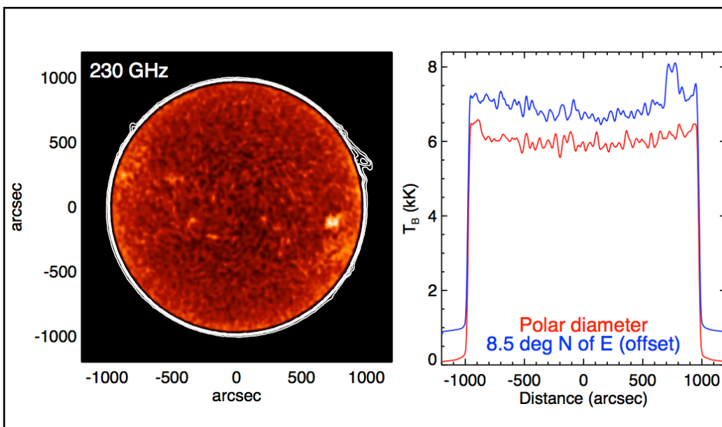
Figure 29: The left panel shows a 230 GHz (band 6) image of the Sun on 7 December 2016. In order to emphasize structure on the disk, the 230 GHz image color display ranges from 5300 to 7400 K. Low-level contours are plotted at 300, 600, 1200, and 2400 K in order to show features above the limb. The right panel shows disk profiles through the Poles and on a diameter through the active region in the southwest quadrant, but with the blue curve offset by 800 K in order to show structure in both. (Credit: ALMA (ESO/NAOJ/NRAO); S. White et al., 2017, SoPh , 292, 88)
