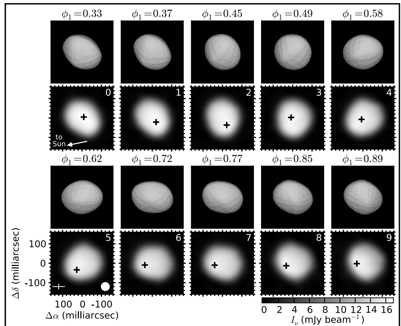
Figure 27: Asteroid 3 Juno was observed in October 2014 during the commissioning period of the ALMA long baseline campaign. Over the course of the observations, the achieved resolution varied from 32 \times 24 mas to 42 \times 36 mas, differing mostly due to changes in phase stability as the observations spanned the transition from night through dawn and into daytime. The baselines used to achieve this resolution ranged from 26 m to 13 km. The observations spanned 10 epochs, covering 60% of the 7.2h rotation period. (Credit: ALMA Partnership et al., 2015, ApJ, 808, L2)
