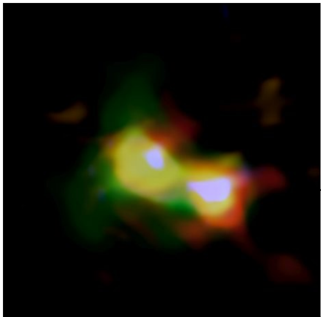
Figure 16: ALMA observed the earliest known example of a merging (non gravitationally lensed) galaxy. This image of B14-65666, a Lyman break galaxy at z=7.15 , shows the distribution of dust (in red), oxygen (in green), and carbon (in blue), observed by ALMA, plus stars (in white) from the HST. (Credits: ALMA (ESO/NAOJ/NRAO), NASA/ESA Hubble Space Telescope, Hashimoto et al., 2019, PASJ , 71, 71)
