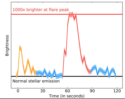
Figure 40: New analysis of ALMA observations reveal that Proxima Centauri emitted a powerful flare that would have created inhospitable conditions for planets in that system. Here is shown the brightness of Proxima Centauri as observed by ALMA over the two minutes of the event on March 24, 2017. The massive stellar flare is shown in red, with the smaller earlier flare in orange, and the enhanced emission surrounding the flare that could mimic a disk in blue. At its peak, the flare increased Proxima Centauri's brightness by 1,000 times. (Credit: M. MacGregor et al., 2018, ApJL , 855, 2)
